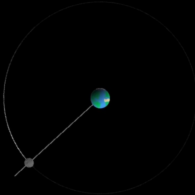
Earth-Moon System
