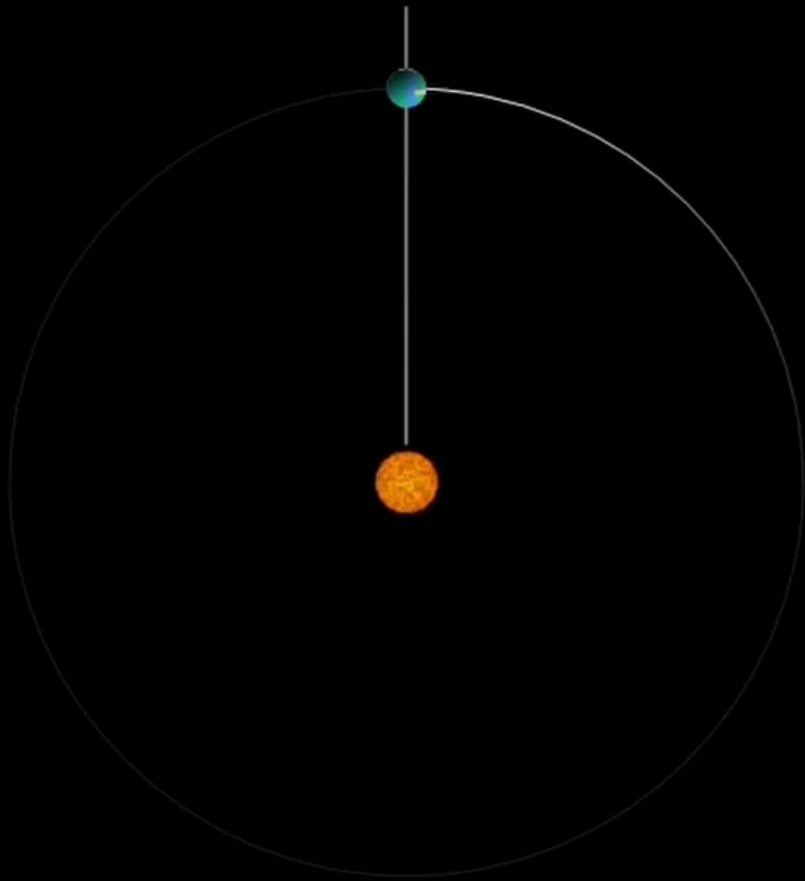
Sun-Earth System
