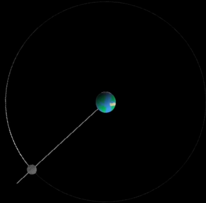
Earth-Moon System
