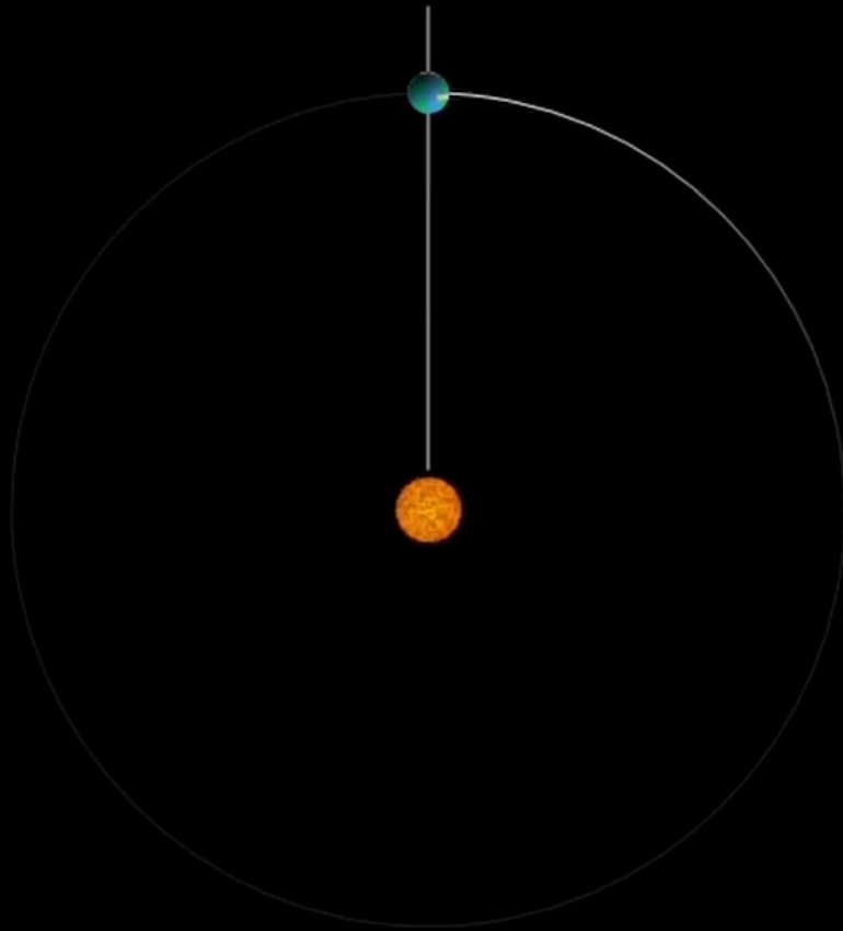
Sun-Earth System
